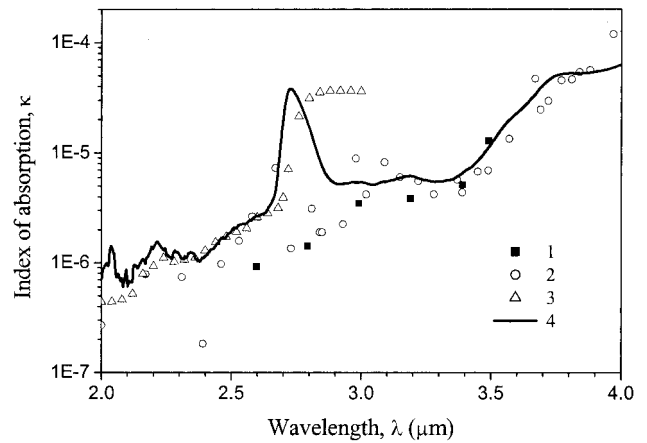
Fig. 5. Comparison of different experimental data for the absorption index of fused quartz: 1, Beder et al. 34 ; 2, Touloukian and DeWitt 35 ; 3, Khashan and Nassif 36 ; 4, present paper.
