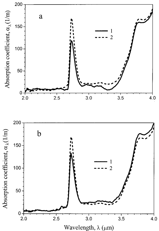
Fig. 9. Absorption coefficient of fused quartz containing bubbles ( f_v = 4\% ): a, z_0 = 5 mm; b, z_0 = 10 mm; 1, experiment; 2, theoretical prediction.
